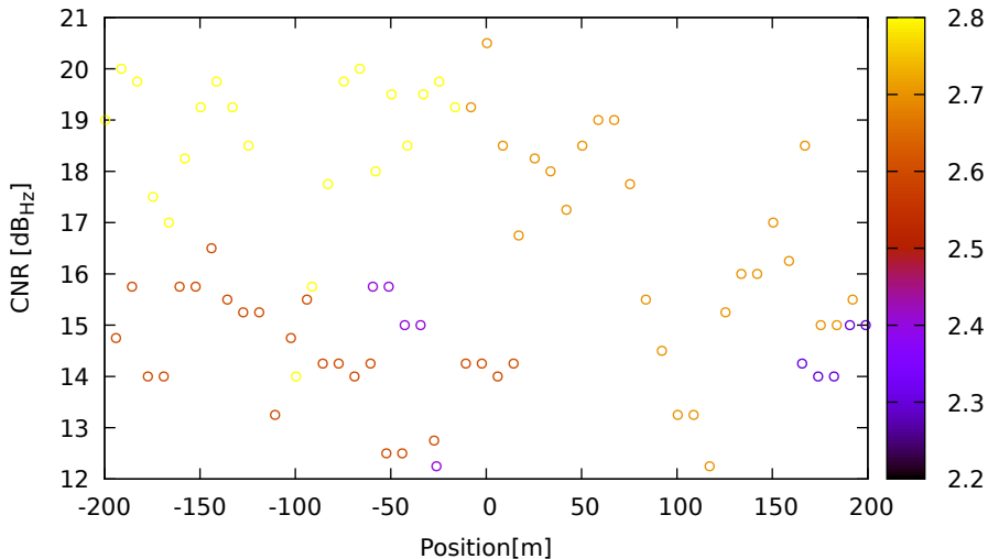
CNR vs position for E27 (E5a) on Xiaomi11T - DOY 262 jam. 2
