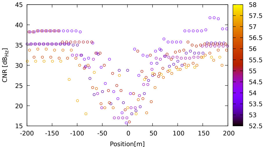
CNR vs position for E34 (E1) on Xiaomi11T - DOY 262 jam. 2
