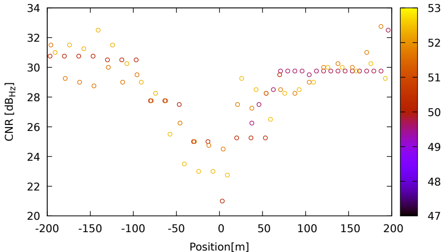
CNR vs position for E34 (E5a) on Xiaomi11T - DOY 262 jam. 1
