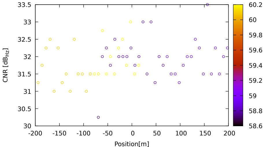
CNR vs position for E34 (E5a) on Xiaomi11T - DOY 262 jam. 3
