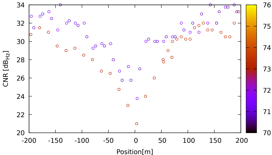
CNR vs position for E36 (E5a) on Xiaomi11T - DOY 262 jam. 1
