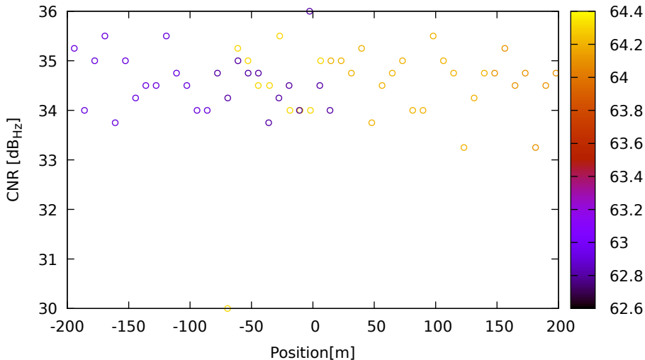
CNR vs position for E36 (E5a) on Xiaomi11T - DOY 262 jam. 3
