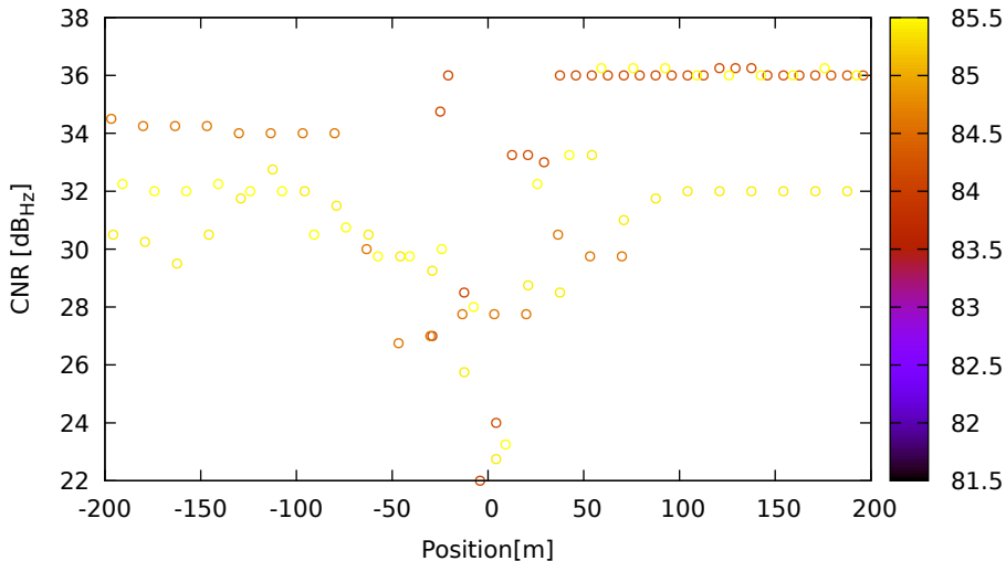
CNR vs position for G01 (L1) on Xiaomi11T - DOY 262 jam. 1
