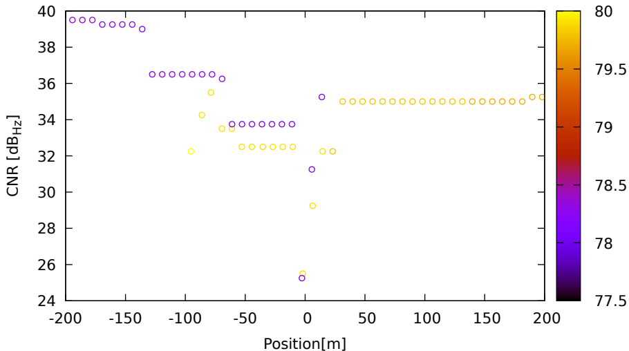
CNR vs position for G01 (L1) on Xiaomi11T - DOY 262 jam. 3
