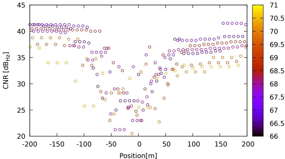
CNR vs position for G03 (L1) on Xiaomi11T - DOY 262 jam. 2
