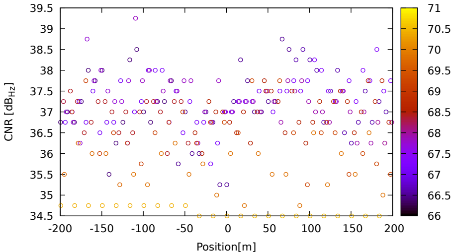
CNR vs position for G03 (L5) on Xiaomi11T - DOY 262 jam. 2
