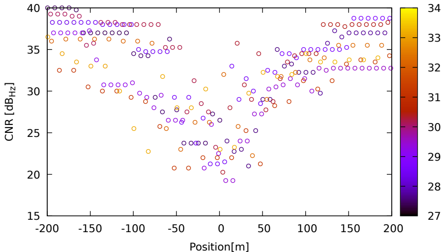
CNR vs position for G04 (L1) on Xiaomi11T - DOY 262 jam. 2
