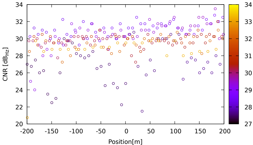
CNR vs position for G04 (L5) on Xiaomi11T - DOY 262 jam. 2
