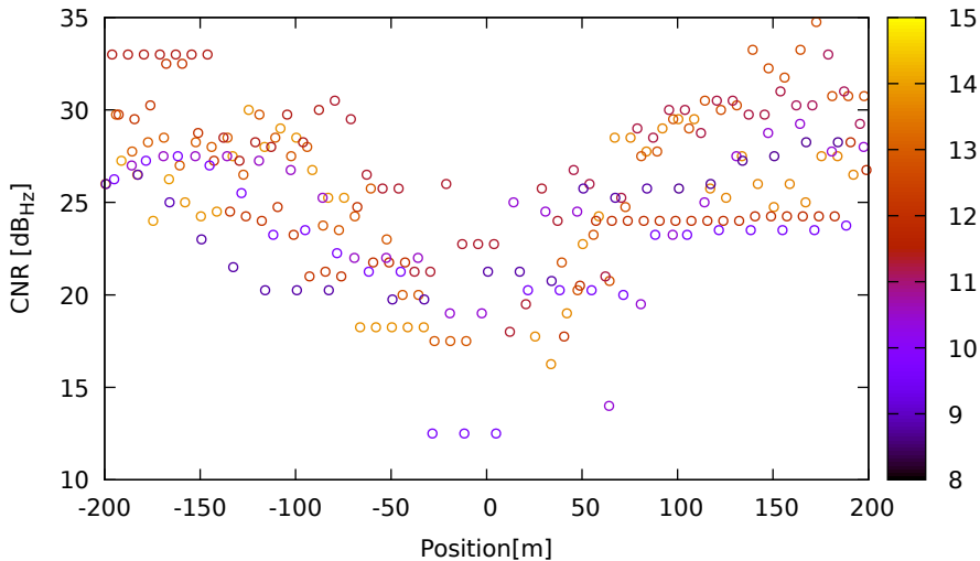
CNR vs position for G08 (L1) on Xiaomi11T - DOY 262 jam. 2
