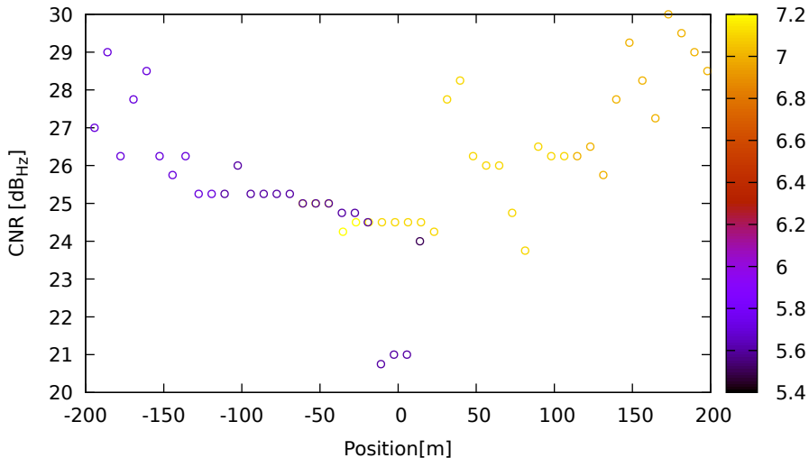
CNR vs position for G08 (L1) on Xiaomi11T - DOY 262 jam. 3
