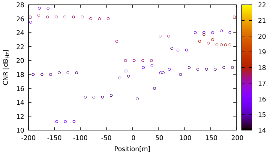
CNR vs position for G08 (L5) on Xiaomi11T - DOY 262 jam. 1
