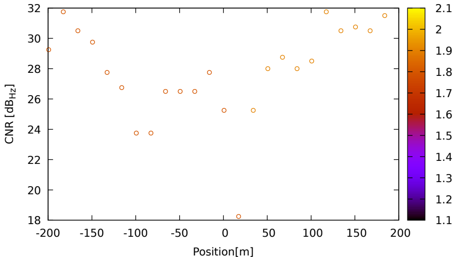
CNR vs position for G09 (L1) on Xiaomi11T - DOY 262 jam. 2
