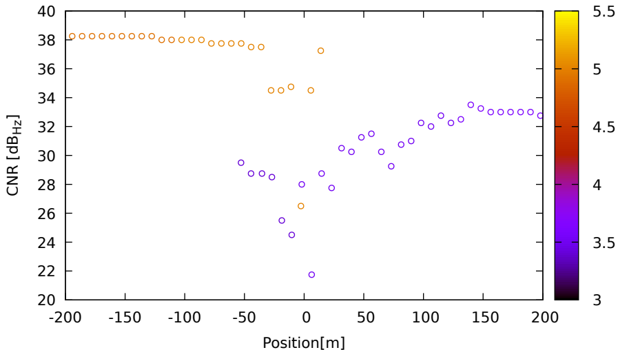
CNR vs position for G09 (L1) on Xiaomi11T - DOY 262 jam. 3
