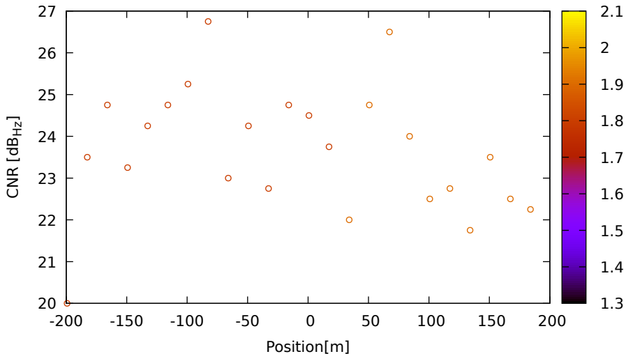
CNR vs position for G09 (L5) on Xiaomi11T - DOY 262 jam. 2
