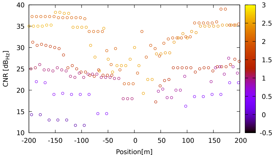
CNR vs position for G14 (L1) on Xiaomi11T - DOY 262 jam. 2
