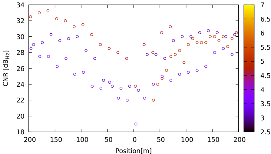
CNR vs position for G14 (L5) on Xiaomi11T - DOY 262 jam. 1
