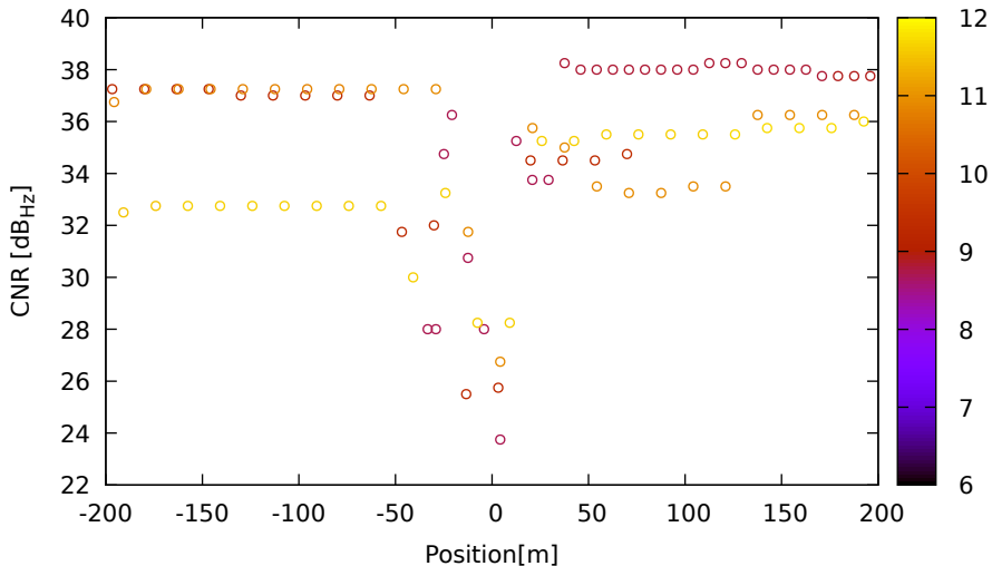
CNR vs position for G19 (L1) on Xiaomi11T - DOY 262 jam. 1
