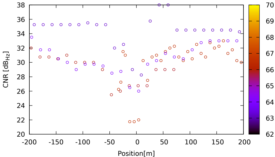
CNR vs position for G21 (L1) on Xiaomi11T - DOY 262 jam. 1
