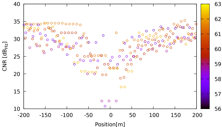
CNR vs position for G21 (L1) on Xiaomi11T - DOY 262 jam. 2
