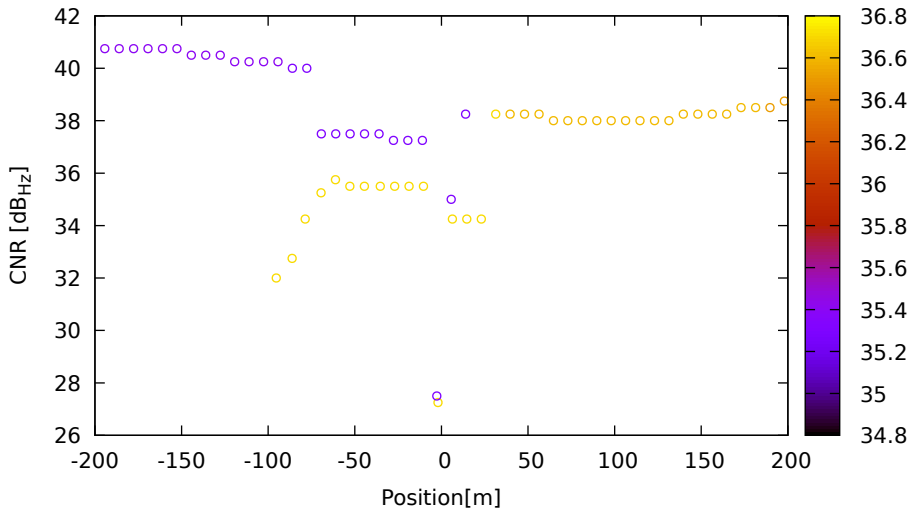
CNR vs position for G22 (L1) on Xiaomi11T - DOY 262 jam. 3
