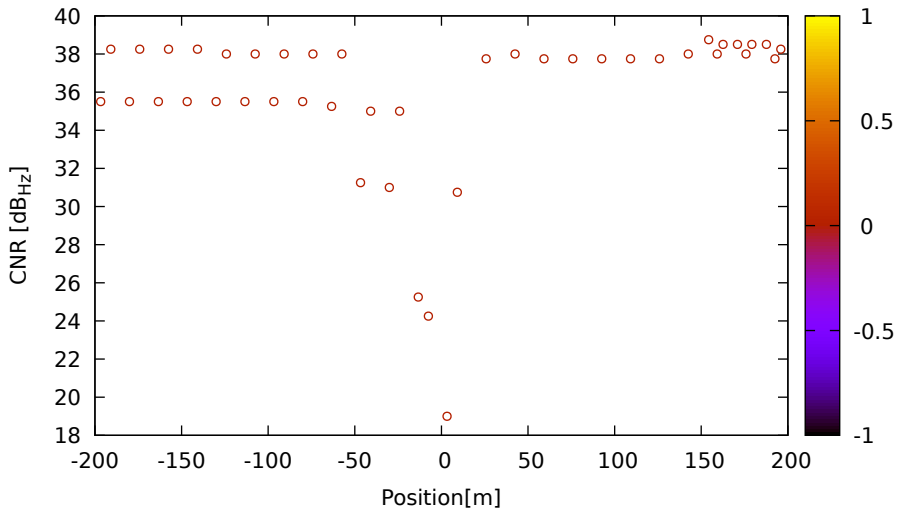
CNR vs position for G28 (L1) on Xiaomi11T - DOY 262 jam. 1
