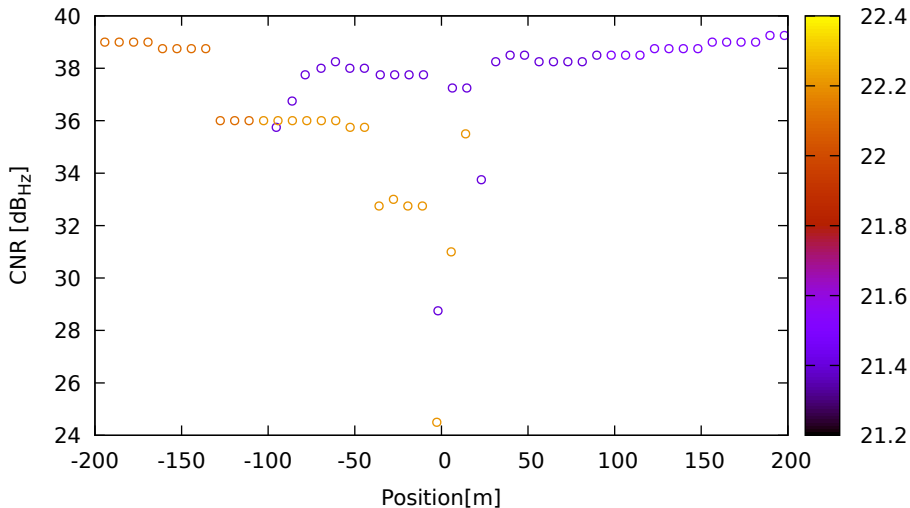
CNR vs position for G31 (L1) on Xiaomi11T - DOY 262 jam. 3
