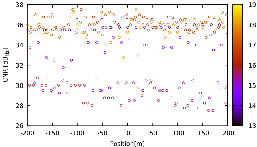
CNR vs position for G32 (L5) on Xiaomi11T - DOY 262 jam. 2
