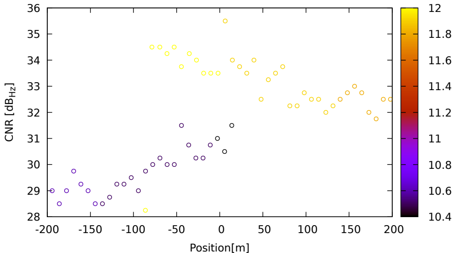
CNR vs position for G32 (L5) on Xiaomi11T - DOY 262 jam. 3
