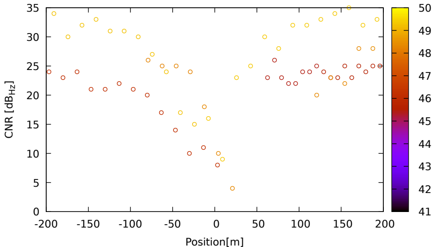
CNR vs position for R01 (G1) on Xiaomi11T - DOY 262 jam. 1
