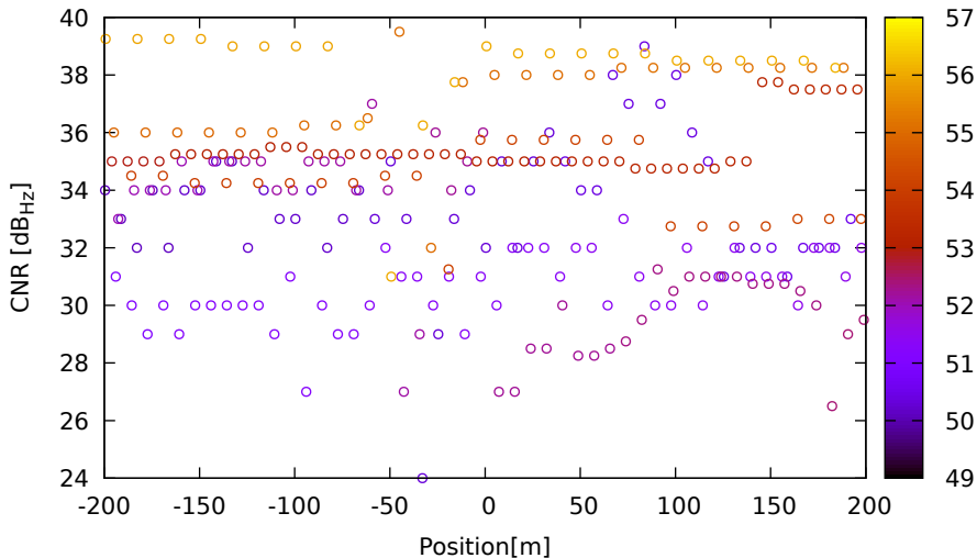
CNR vs position for R01 (G1) on Xiaomi11T - DOY 262 jam. 2
