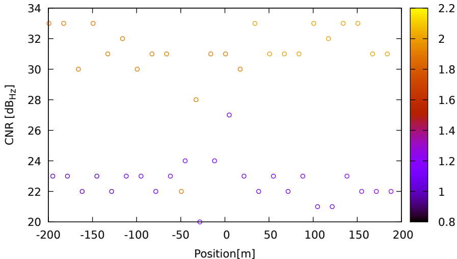
CNR vs position for R02 (G1) on Xiaomi11T - DOY 262 jam. 2
