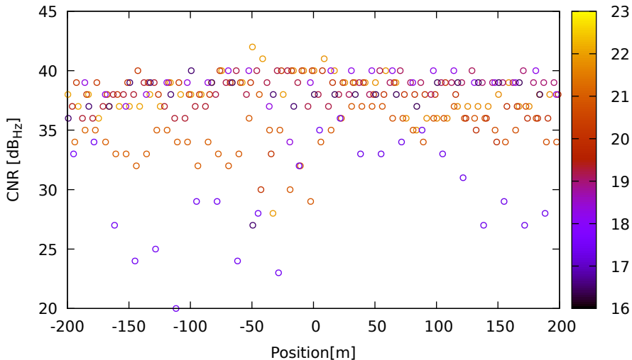
CNR vs position for R07 (G1) on Xiaomi11T - DOY 262 jam. 2
