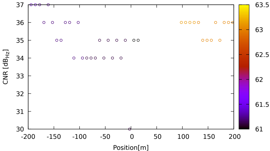
CNR vs position for R08 (G1) on Xiaomi11T - DOY 262 jam. 3
