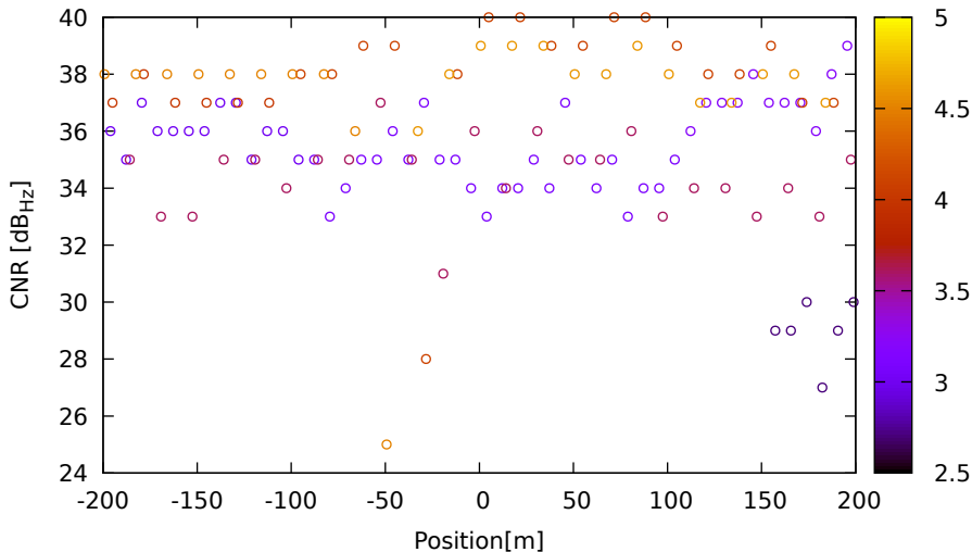
CNR vs position for R09 (G1) on Xiaomi11T - DOY 262 jam. 2
