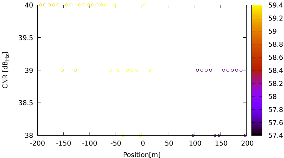
CNR vs position for R24 (G1) on Xiaomi11T - DOY 262 jam. 3
