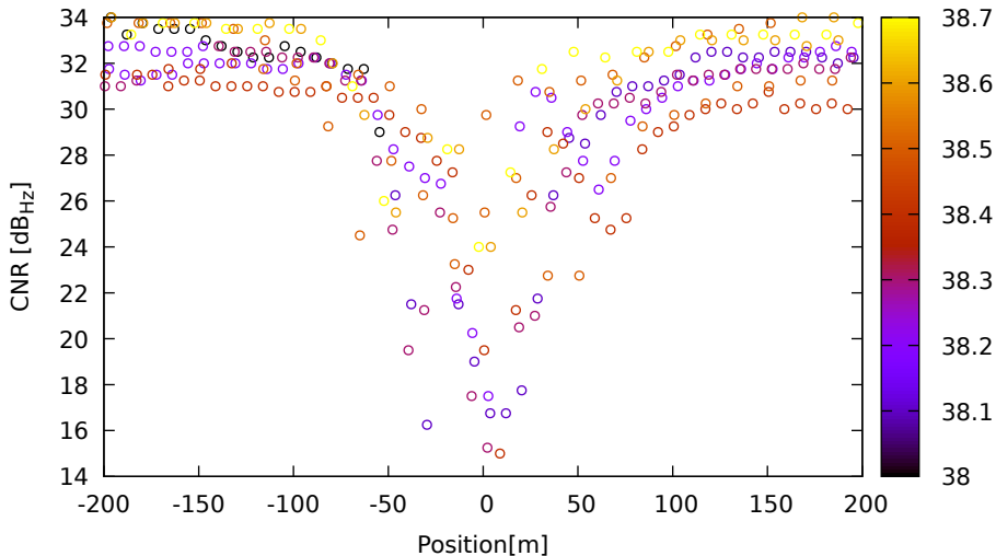
CNR vs position for C09 (B1) on XiaomiMi8 - DOY 262 jam. 2
