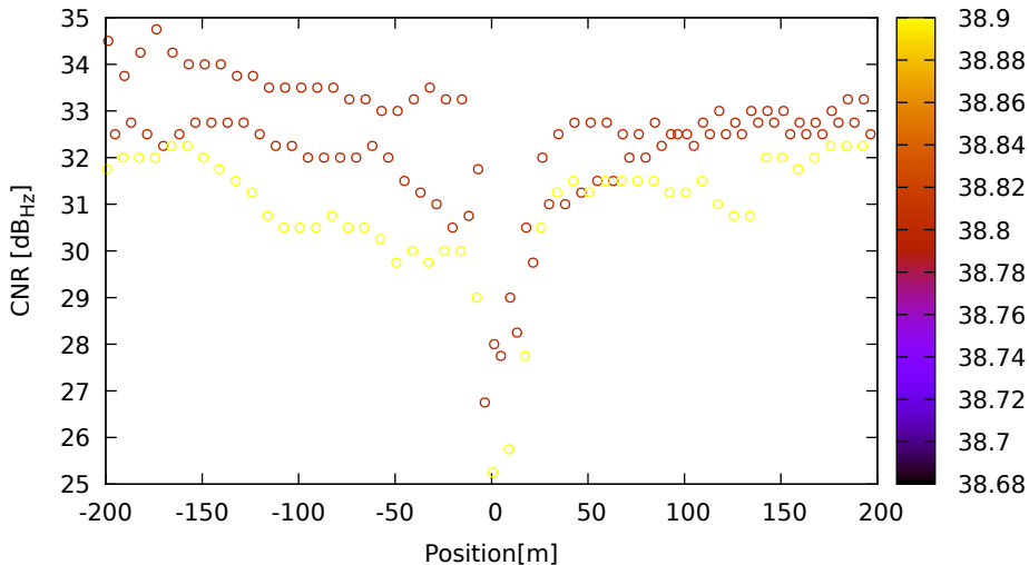
CNR vs position for C09 (B1) on XiaomiMi8 - DOY 262 jam. 3
