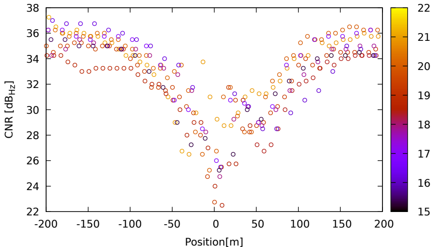
CNR vs position for C11 (B1) on XiaomiMi8 - DOY 262 jam. 1
