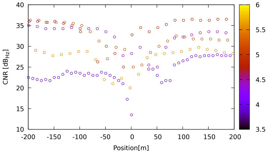
CNR vs position for C26 (B1) on XiaomiMi8 - DOY 262 jam. 2
