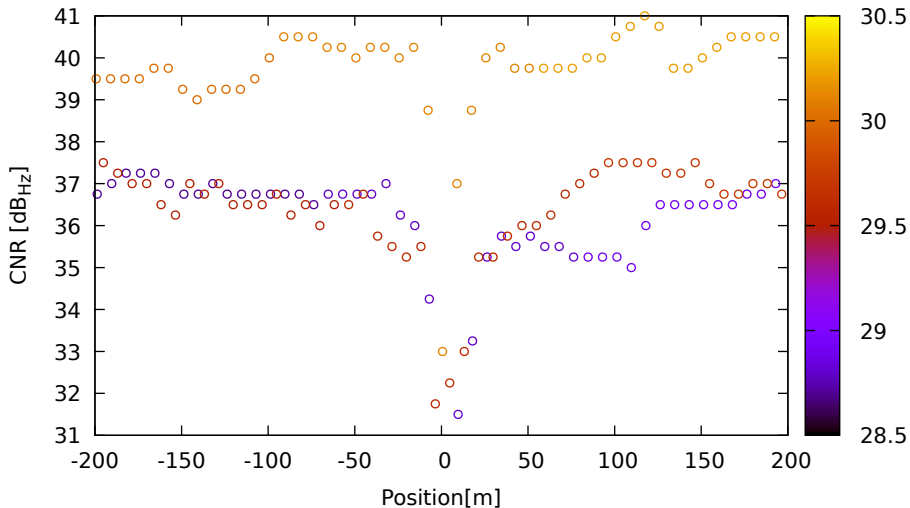
CNR vs position for C27 (B1) on XiaomiMi8 - DOY 262 jam. 3
