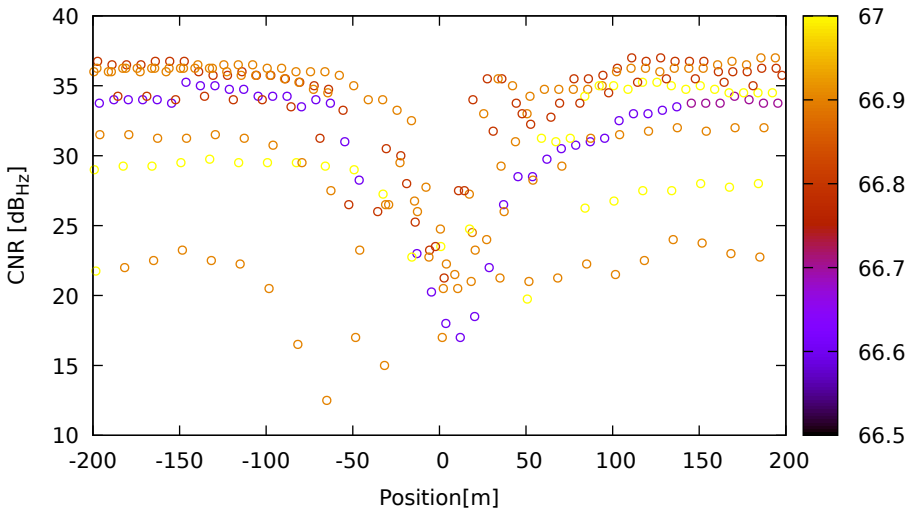
CNR vs position for C28 (B1) on XiaomiMi8 - DOY 262 jam. 2
