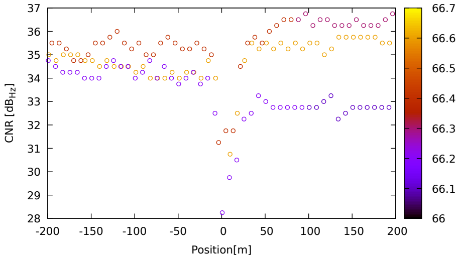
CNR vs position for C28 (B1) on XiaomiMi8 - DOY 262 jam. 3
