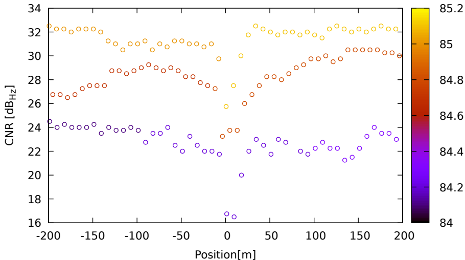
CNR vs position for C33 (B1) on XiaomiMi8 - DOY 262 jam. 3
