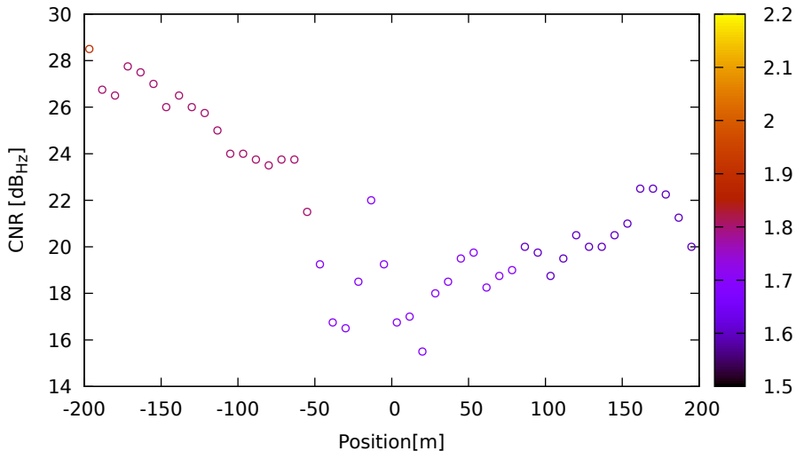
CNR vs position for C34 (B1) on XiaomiMi8 - DOY 262 jam. 1
