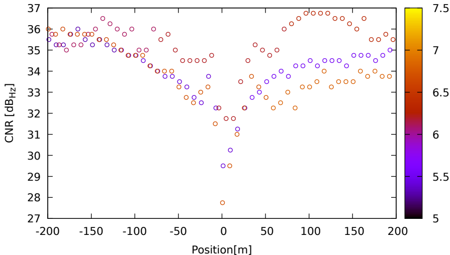
CNR vs position for E03 (E1) on XiaomiMi8 - DOY 262 jam. 3
