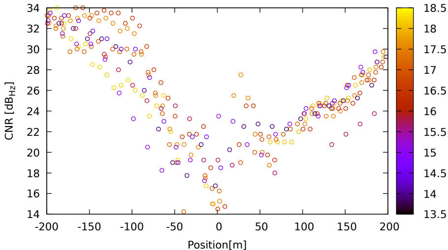
CNR vs position for E04 (E1) on XiaomiMi8 - DOY 262 jam. 2
