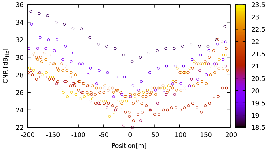
CNR vs position for E04 (E5a) on XiaomiMi8 - DOY 262 jam. 1
