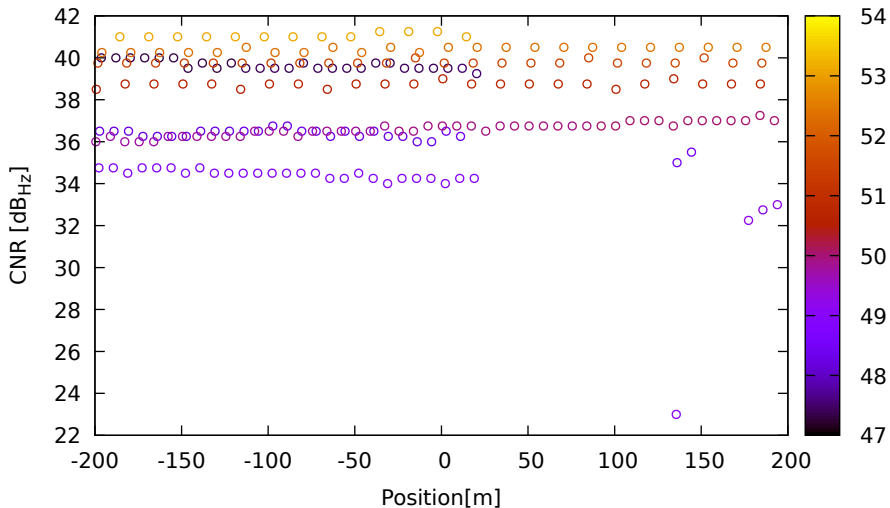
CNR vs position for E05 (E5a) on XiaomiMi8 - DOY 262 jam. 2
