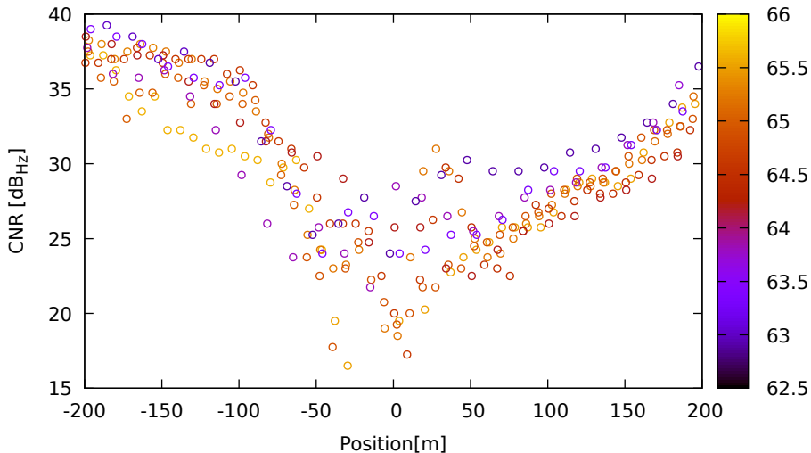
CNR vs position for E09 (E1) on XiaomiMi8 - DOY 262 jam. 2
