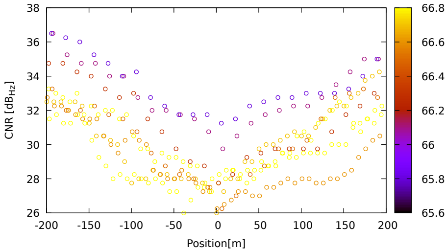
CNR vs position for E09 (E5a) on XiaomiMi8 - DOY 262 jam. 1
